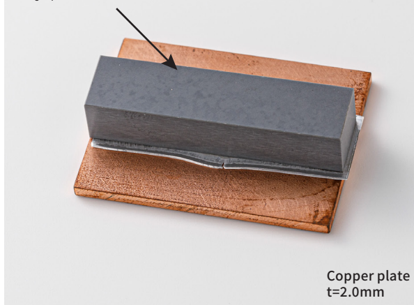
Silicon Nitride Block & Copper Plate
