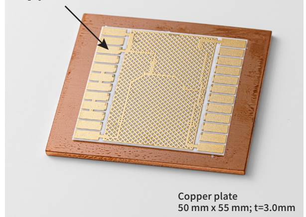
Alumina Substrate & Copper Plate
