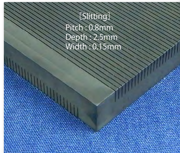
[Whole sample] □ 50.0mm/6.5mm thick
