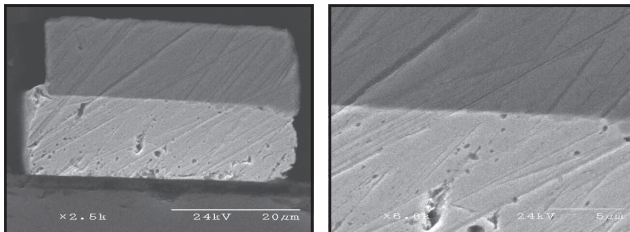
(Magnified bonded cross section)
