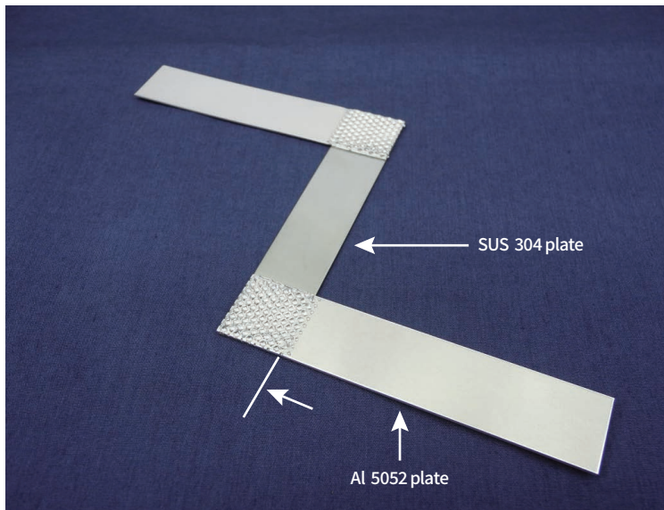
Bending test
