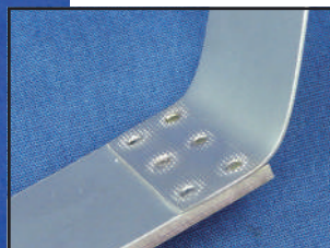
上側 SUS304 (t=0.5mm) 下側 SUS304 (t=2mm)
