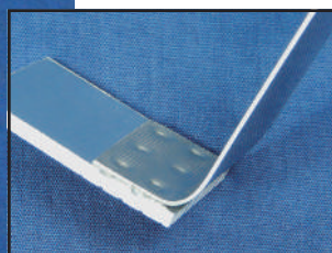
上側 SUS304 (t=0.5mm) 下側 Aluminum (t=2mm)
