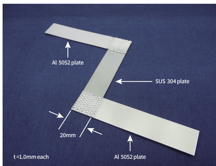
Bending test
