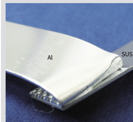
Bending test
