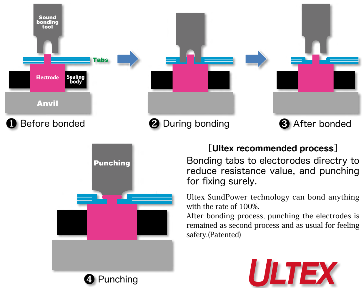
Bonding of Aluminum tabs to Aluminum electrodes directly
