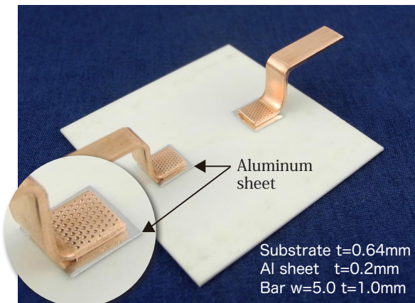
★ [Alumina substrate & Copper bars] Bonding by sandwiching Aluminum sheet
