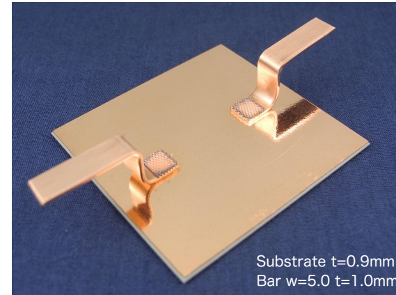
★ [AMC substrate & Copper bars]
