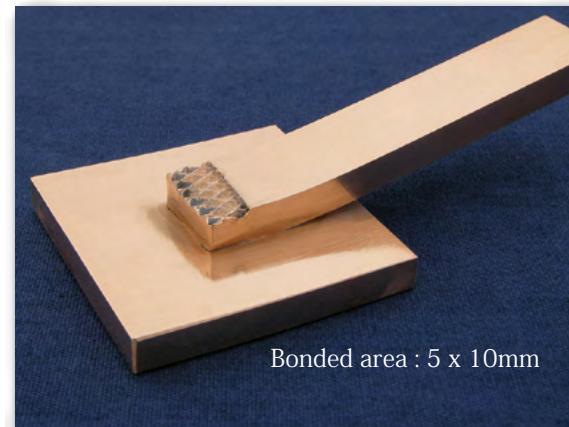
★ [Thickness 4mm] Copper bar & Copper block
