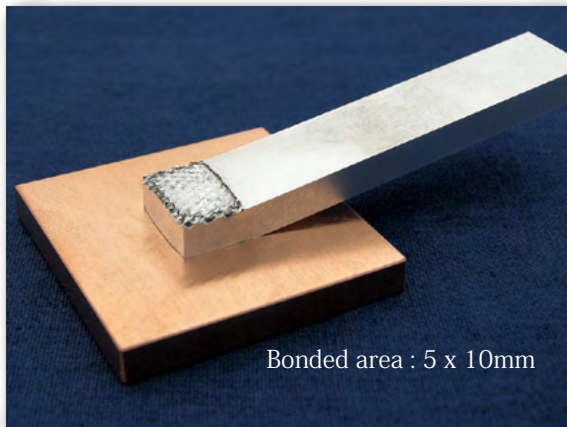
★ [Thickness 4mm] Aluminum bar & Copper block
